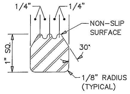
RUNG DETAIL
